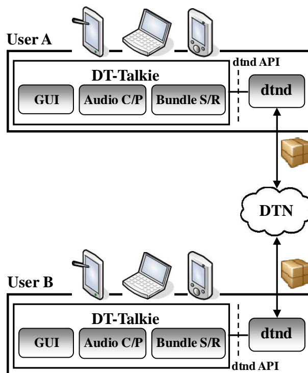
Figure 1: DT-Talkie Architecture
